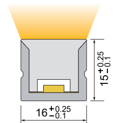
Unit: mm Cross section
