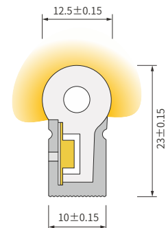
Unit: mm Cross section
