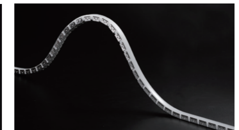
Stainless Flexible Profile Item No.: JK0021 Dimension (LxWxH): 970x16x16.3mm Material: SUS304\SUS316
