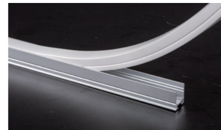
Aluminum Profile Item No.: JA0049 Dimension(LxWxH): 1000x19x21.5mm Material: Aluminum
