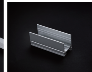
Aluminum Clips Item No.: JA0049 Dimension(LxWxH): 30X19X21.5mm 50X19X21.5mm Material: Aluminum 6063
