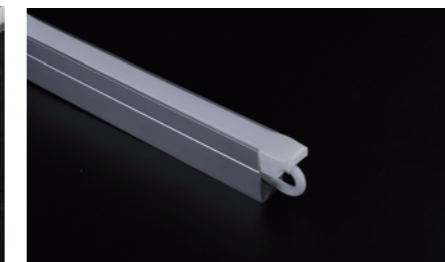
Aluminum Profile (Outlet) Item No.: JA0105 Dimension (LxWxH): 1000x21x41.5mm Material: Aluminum
